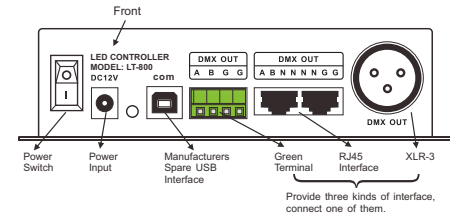
Controller (Receiver)
